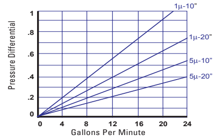
Full-Flow (BB) Cartridge
